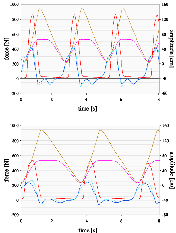
Figure 1: Grip amplitude (light red), seat amplitude (pink), grip force (dark red) and foot rest forces of the left (light blue) and right foot (dark blue) during slow (top) and fast (bottom) rowing cycles.
