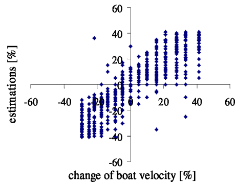
Figure 2: Correlation of estimated and calculated virtual boat velocity of an indoor rower.
