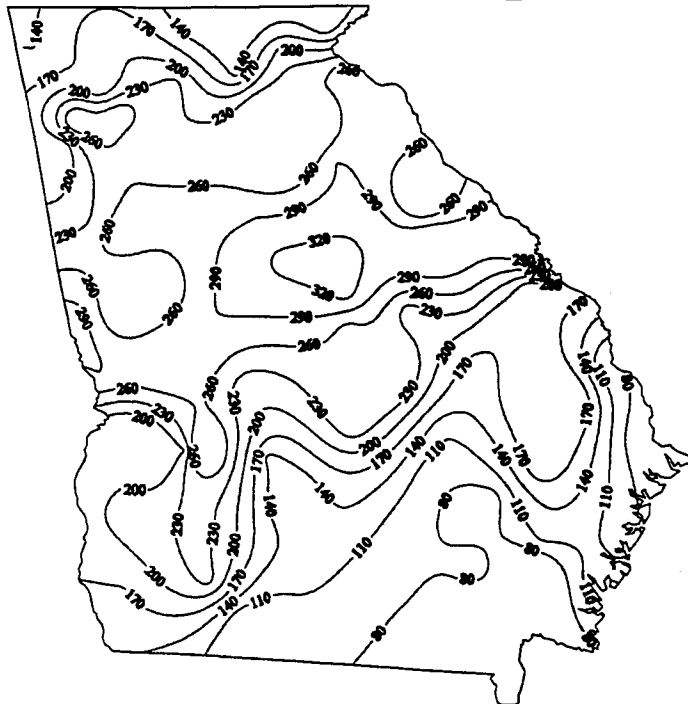
Figure 6. Spatial distribution of irrigation requirements (in mm) for maize and soybean growth, development and yield formation, averaged for the period 1961-1990.
