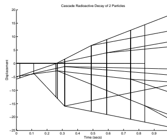
Figure 3: A Cascading Radioactive Decay
