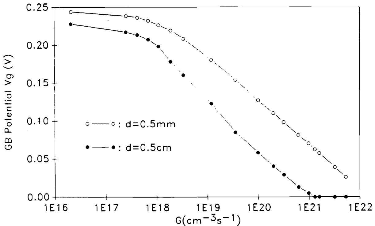
Fig.1 V_g as a function of generation rate for p-type poly-Si at N_a=1\text{E}16(\text{cm}^{-3}) , N_{ts}=5\text{E}12(\text{cm}^{-2}) .
