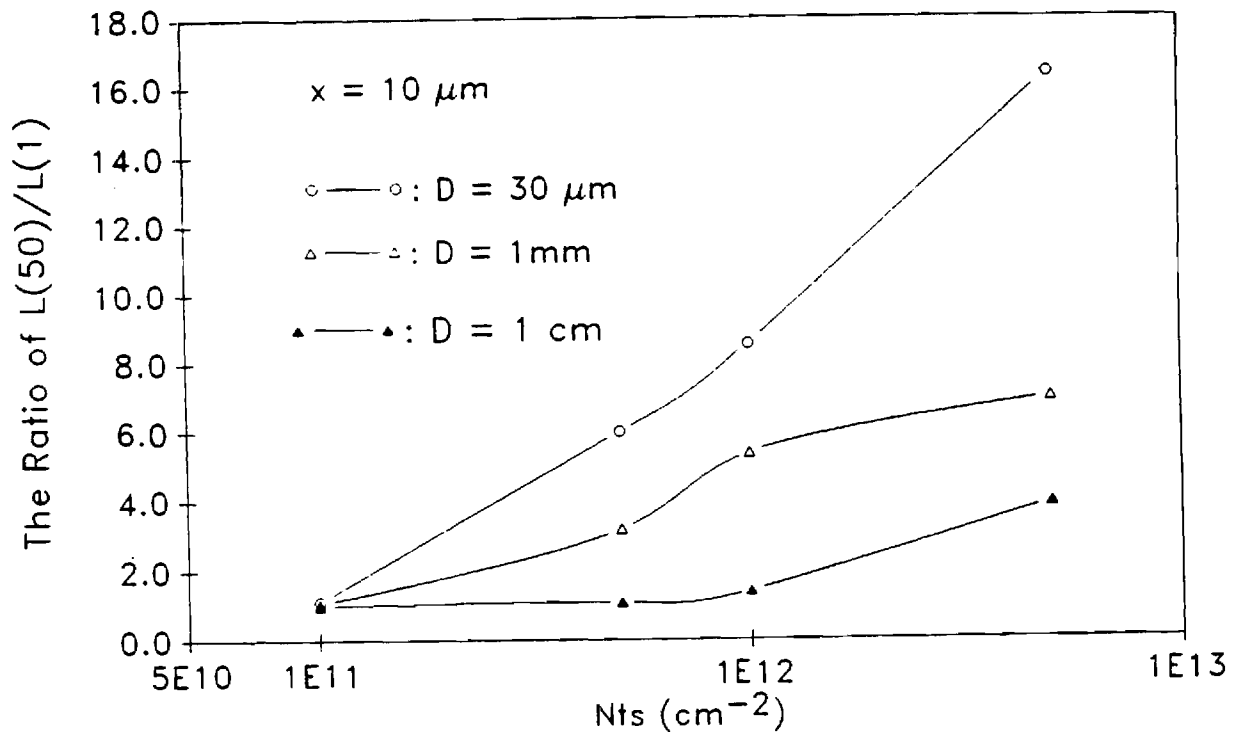
Fig.3 The effects of N_{ts} and D on the ratio of L(50)/L(1) .
