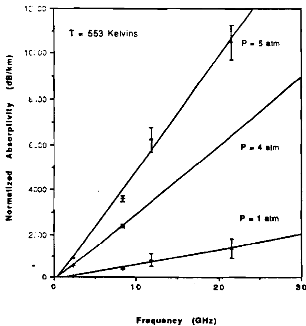
H2SO4 Opacity Data
