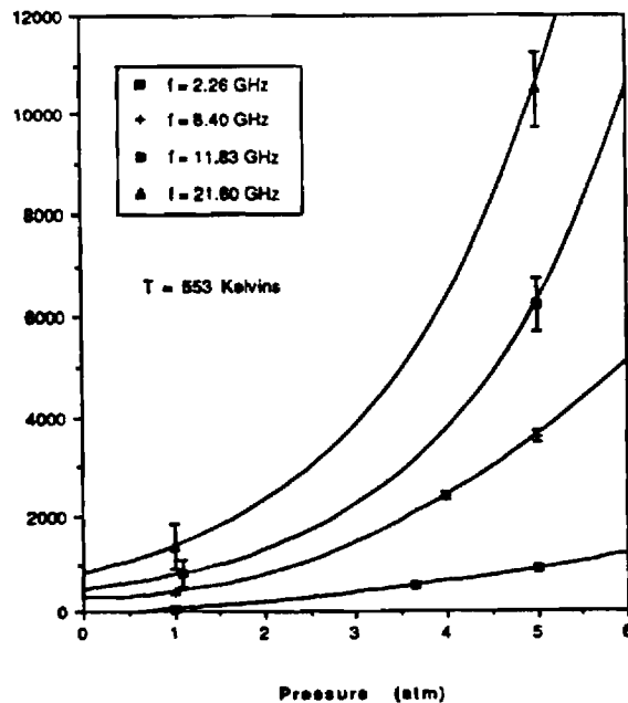
H2SO4 Opacity Data
