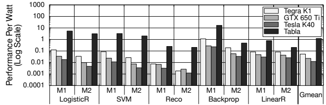
(a) Performance-per-Watt comparison between ARM, Xeon and TABLA. (b) Performance-per-Watt comparison between Tegra, GTX 650, Tesla and TABLA
