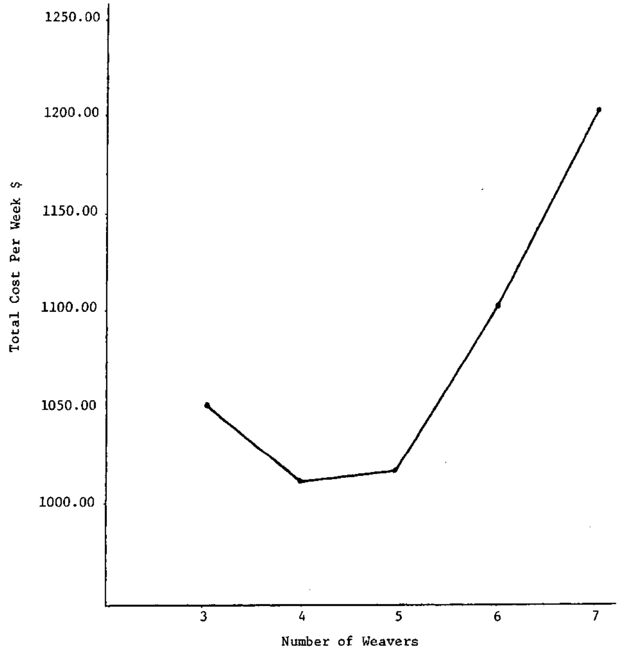
Figure 5. Total Cost vs. the Number of Weavers
